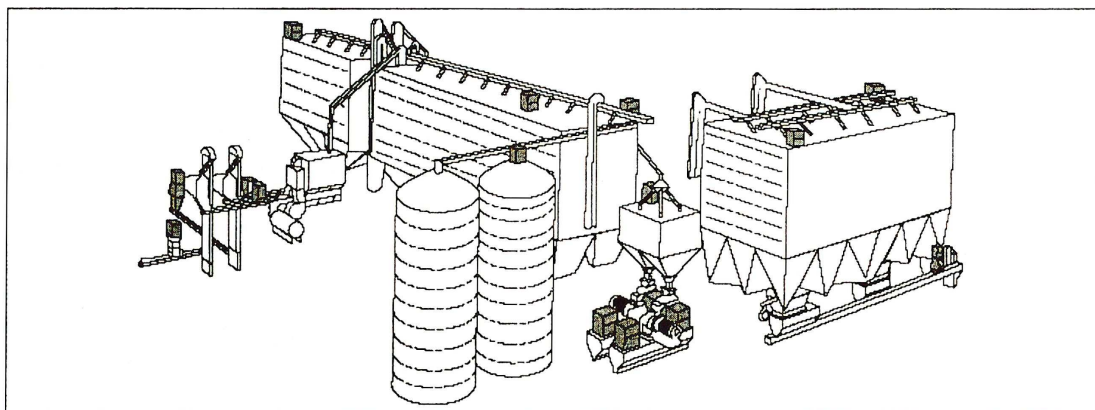
Figure 10 a) Central Dust Collection System; b) Integrated Dust Collection System; c) Unit Dust Collection System
